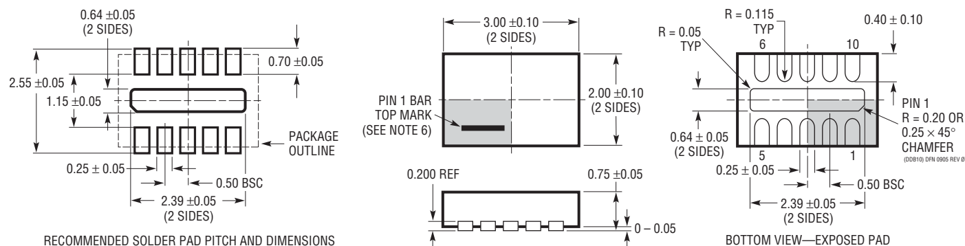
DDB Package 10-Lead Plastic DFN (3mm × 2mm) (Reference LTC DWG # 05-08-1722 Rev 0)
